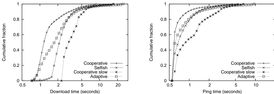
Figure 3: Cumulative download and ping time with the gold star scheme and no background traffic.
