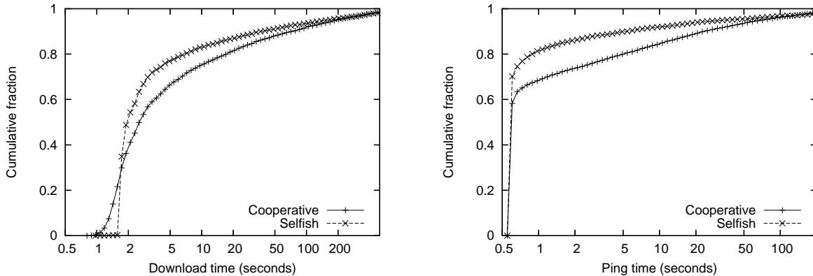
Figure 7: Cumulative download and ping time with the pair-wise reputation design and heavy traffic (20 BitTorrent clients and 2000 web clients). Four relay types (cooperative, selfish, cooperative reserve, and adaptive) are simulated, although only the performance of the former two are shown, as the latter two behave similarly to cooperative relays.
