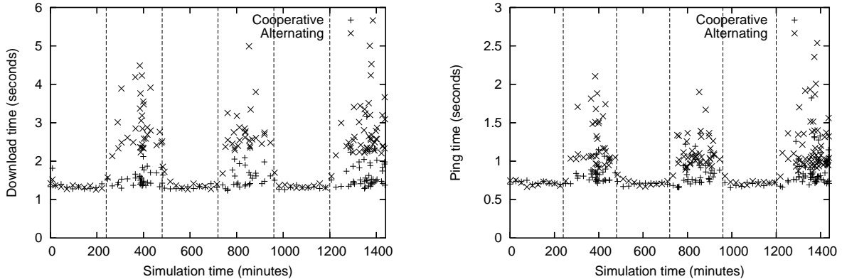
Figure 6: Average download and ping time with relays that alternate between being cooperative and selfish. This experiment is with the gold star scheme in place and heavy background traffic (20 BitTorrent clients and 2000 web clients). Dotted lines show the times at which the alternating relays switch. The performance of alternating relays gets worse whenever they switch to being selfish, while performance for cooperative relays only suffers a little.
