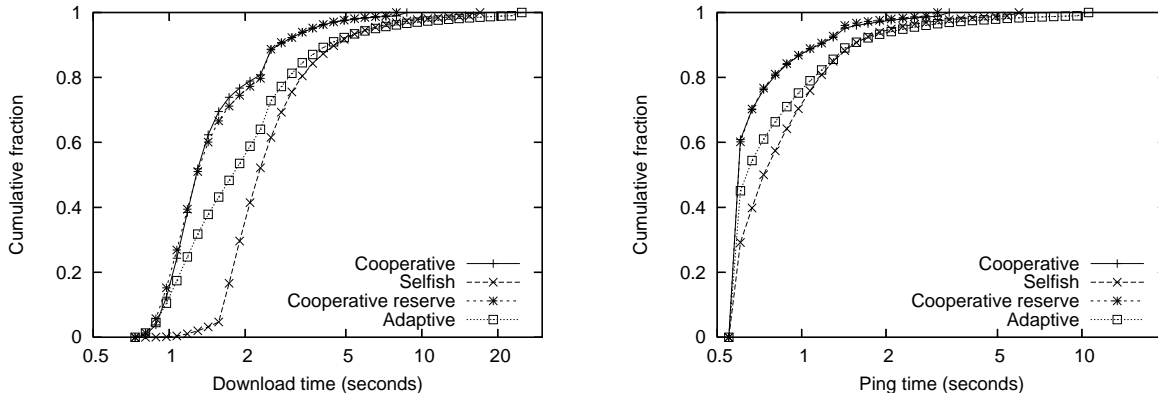
Figure 5: Cumulative download and ping time with the gold star scheme and heavy background traffic (20 BitTorrent clients and 2000 web clients). Cooperative reserve relays, which replaced the cooperative slow relays, have similar performance to fully cooperative relays.
