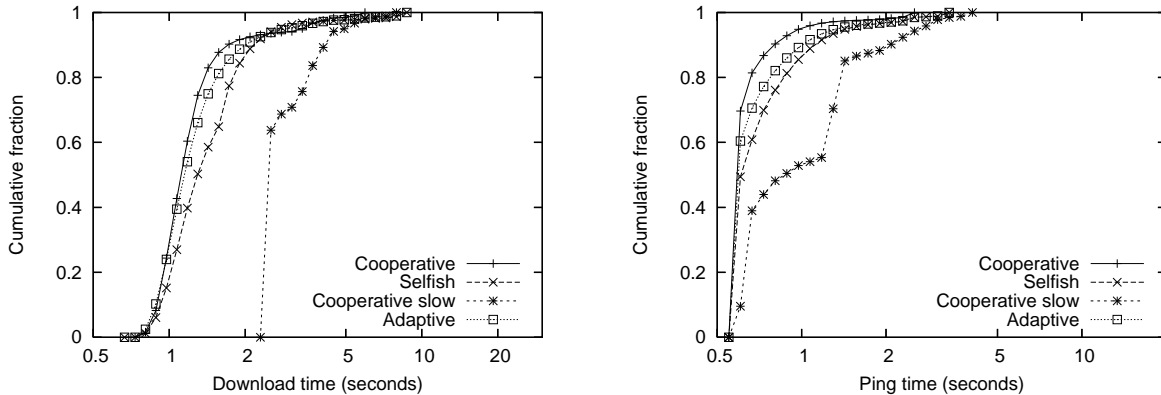
Figure 3: Cumulative download and ping time with the gold star scheme and no background traffic.
