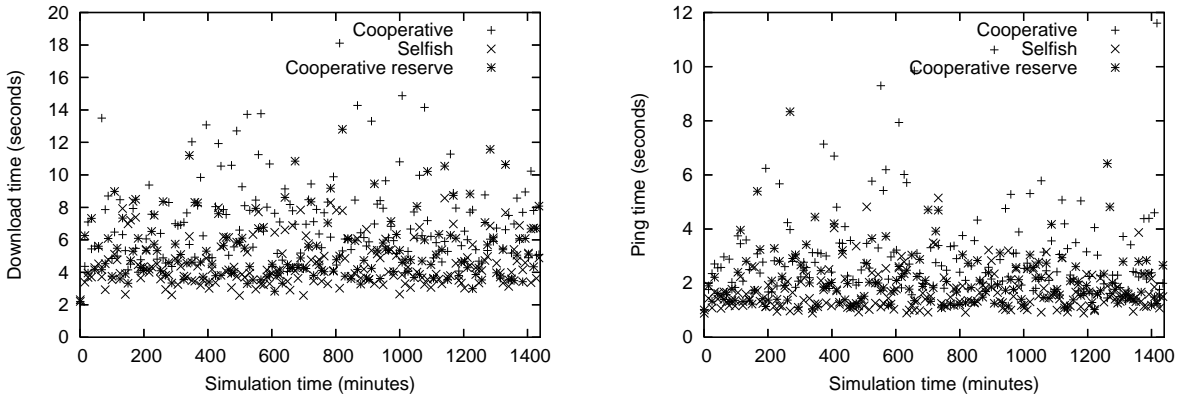
Figure 1: Average download and ping time over time when no incentive scheme is in place and heavy traffic (20 BitTorrent clients and 2000 web clients). Both download and ping time show significant variation, regardless of relay type.
