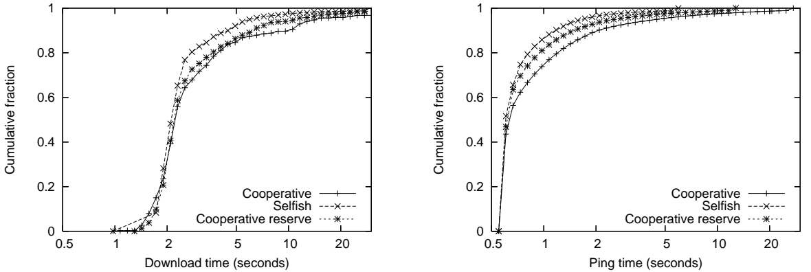
Figure 2: Cumulative download and ping time when no incentive scheme is in place and heavy traffic (20 BitTorrent clients and 2000 web clients). Performance for all relay types is similar, although selfish relays do somewhat better in the worst case.
